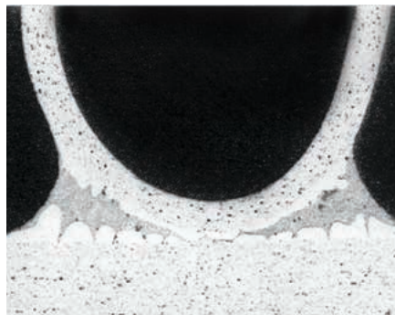
Back side of flat tube has improved heat transfer, reduced pressure drop with lower noise.
