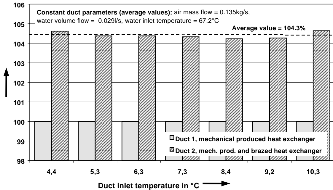
Deviation of capacity transfer (water side) in %, base: values of duct 1 = 100%
