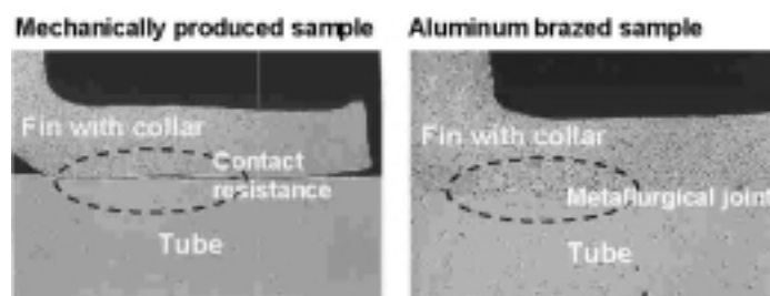
Figure 1: Microscopic surfaces of a mechanical produced and aluminum brazed joint sample [5]
