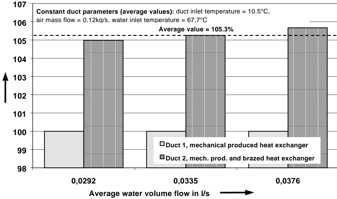
Figure 4: Short term test, capacity transfer on the water side for different average water volume flows and heat exchangers
