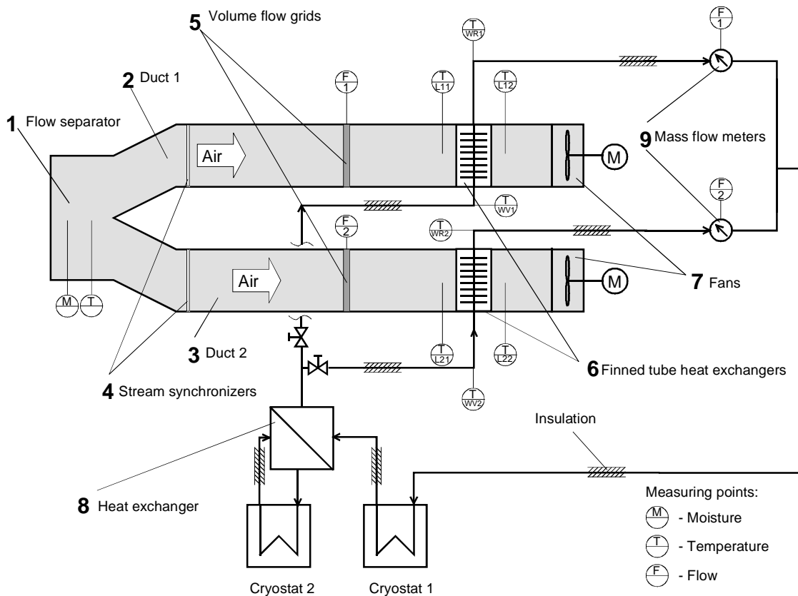
Figure 2: Test facility
