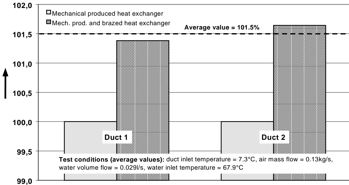
Figure 5: Comparison of the average capacity transfer of different heat exchangers in duct 1 and 2 from both long term tests
